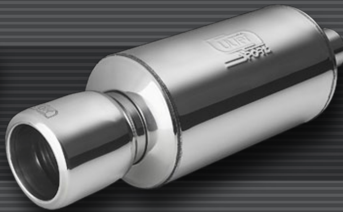
NRS-001/16-1 (length 250mm, diameter 150mm) NRS-002/16-1 (length 330mm, diameter 150mm)
